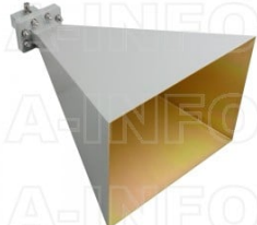
LB-187-20-C-TF Standard Gain Horn Antenna 3.95-5.85GHz 20dB Gain TNC Female
